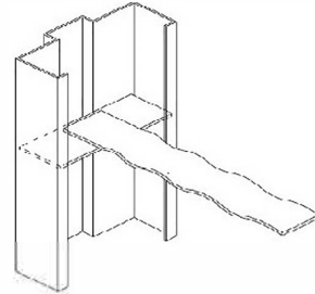
MASONRY STRAPS
