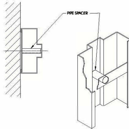
TUBE SUPPORTS
