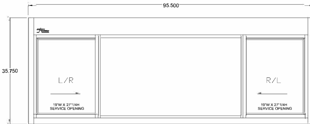
MODEL 550 - 95 1/2 X 35 3/4 H OUTSIDE VIEW
