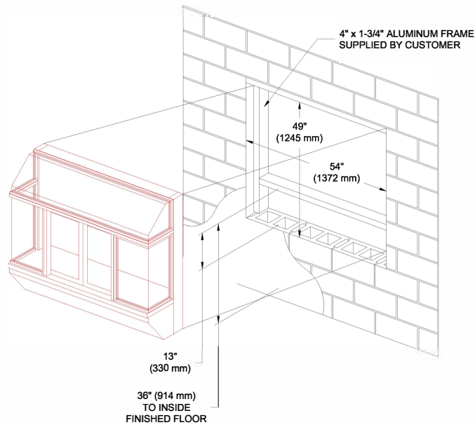
MASONRY WALL ROUGH OPENING
