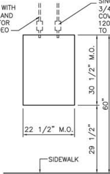
WALL OPENING EXTERIOR ELEVATION
