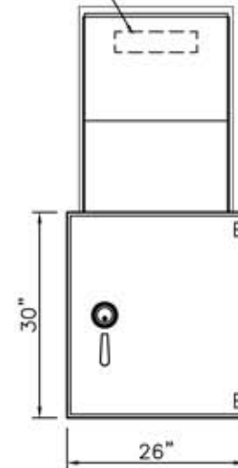
INTERIOR ELEVATION
