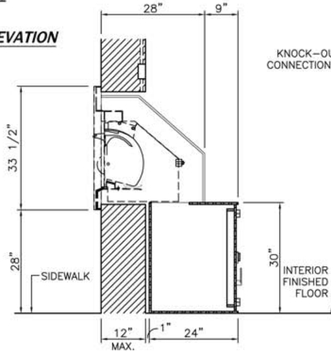
DEPOSITORY ASSEMBLY VERTICAL SECTION
