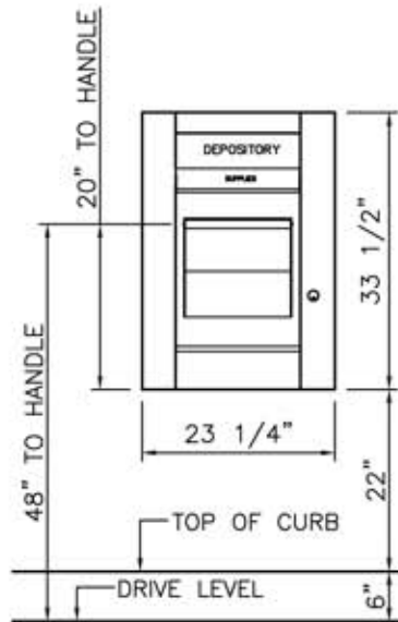
EXTERIOR ELEVATION
